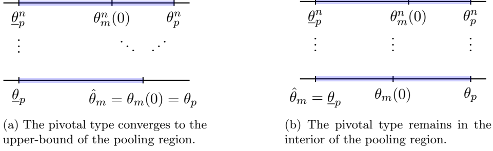
Figure B.1: Implications of Definition B.3. Suppose that b_m^n(\underline{\theta}_p) = b_m^n(\theta_m^n(0)) = b_m^n(\theta_p^n) along some sequence. In subfigure (a), \theta_m(0) = \lim \theta_p^n and therefore \hat{\theta}_m = \theta_m(0) . In subfigure (b) \theta_m(0) < \lim \theta_p^n and therefore \hat{\theta}_m = \lim \underline{\theta}_p^n .
